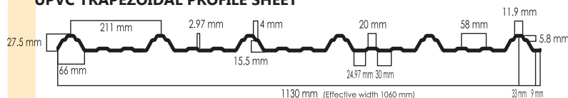
UPVC TRAPEZOIDAL PROFILE SHEET
